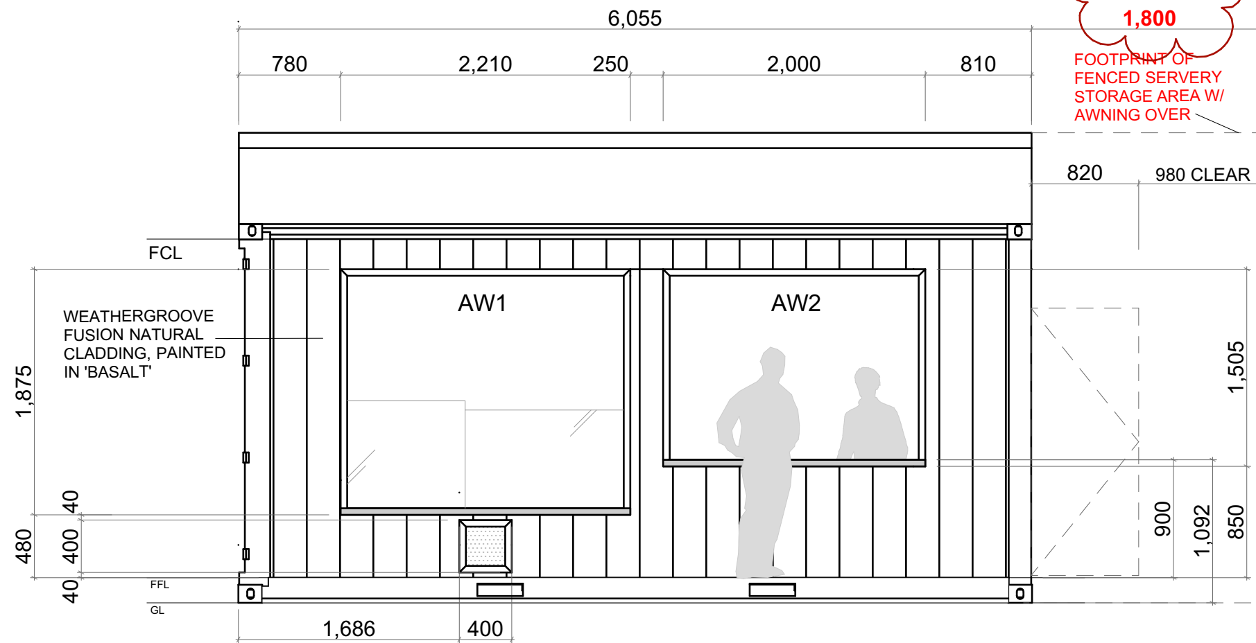
FRONT ELEVATION
