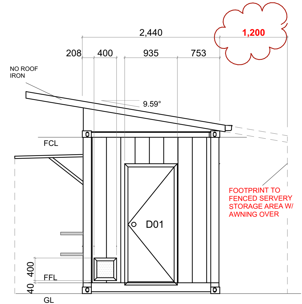
SIDE ELEVATION
