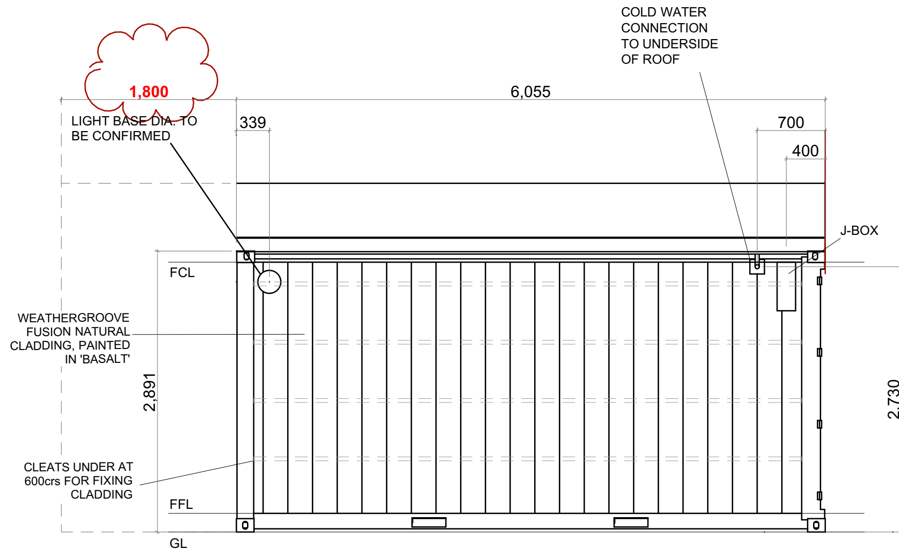
REAR ELEVATION
