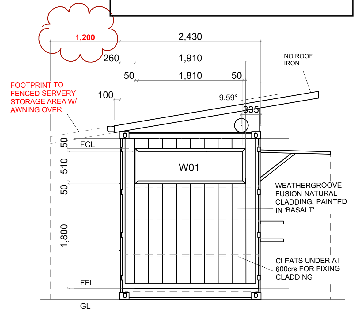
SIDE ELEVATION
